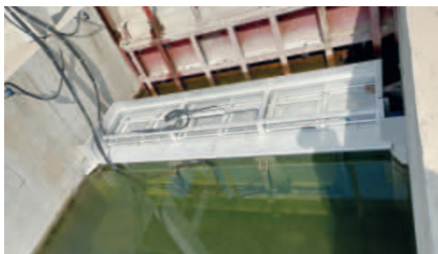
Figure 10 Drainage of the overflow structure and preparing of the assembly (top); finished system consisting of hydraulically driven raked bar screen and flushing gate below waterline (bottom)
